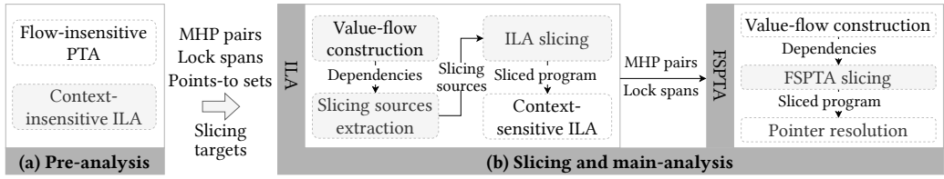
Fig. 1. Framework overview of multi-stage slicing.
