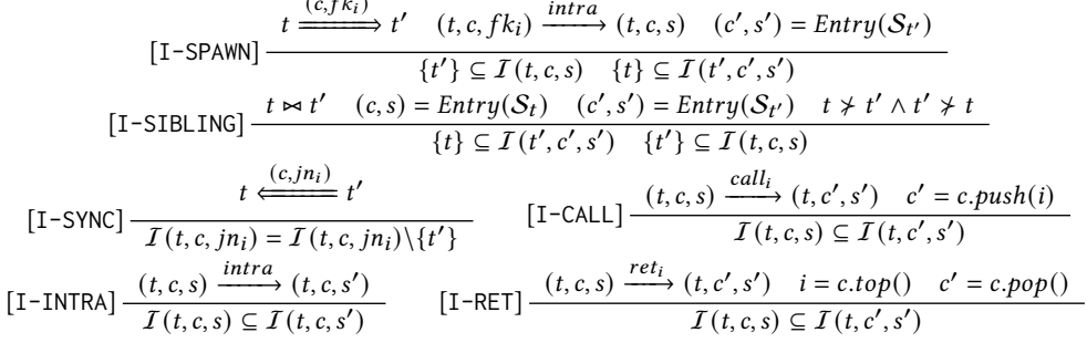
Fig. 3. Inference rules for interleaving analysis [39].
